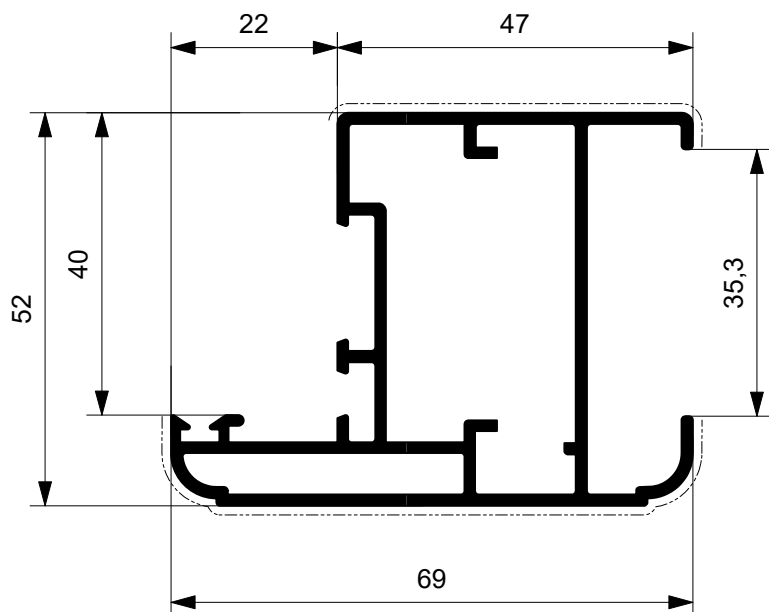
R 6653 Kg/ml 1.220 --- mm. 145
