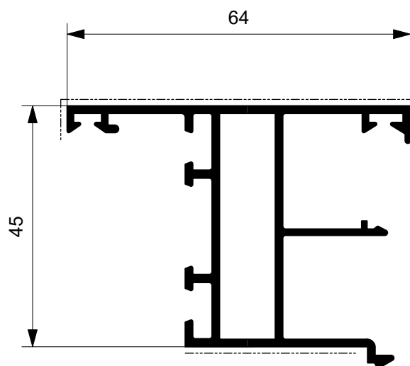
M 9250 Kg/ml 0.956 --- mm. 74
