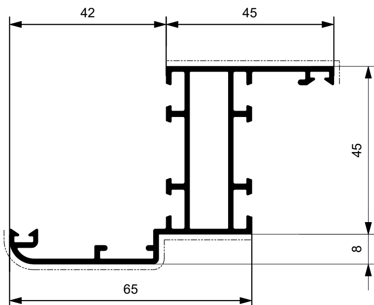
M 8427 Kg/ml 1,037 --- mm. 127
