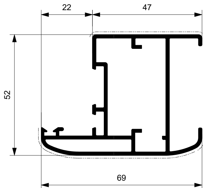
R 6654 Kg/ml 1.208 --- mm. 145
