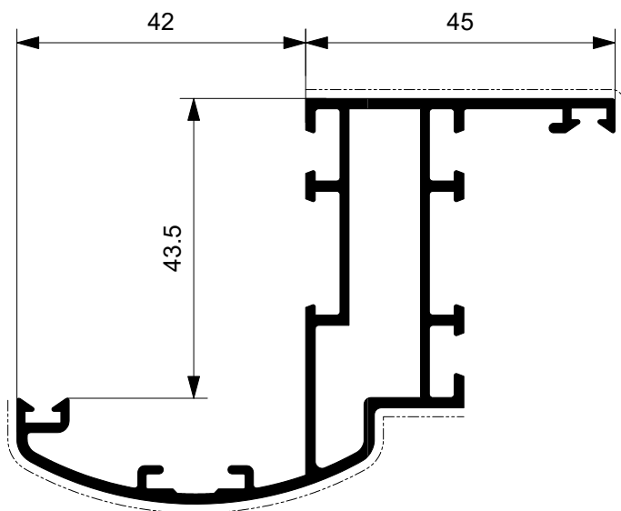
R 5256 Kg/ml 1.120 --- mm. 133
