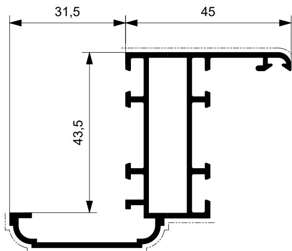
CM 5480 Kg/ml 1.010 --- mm. 119
